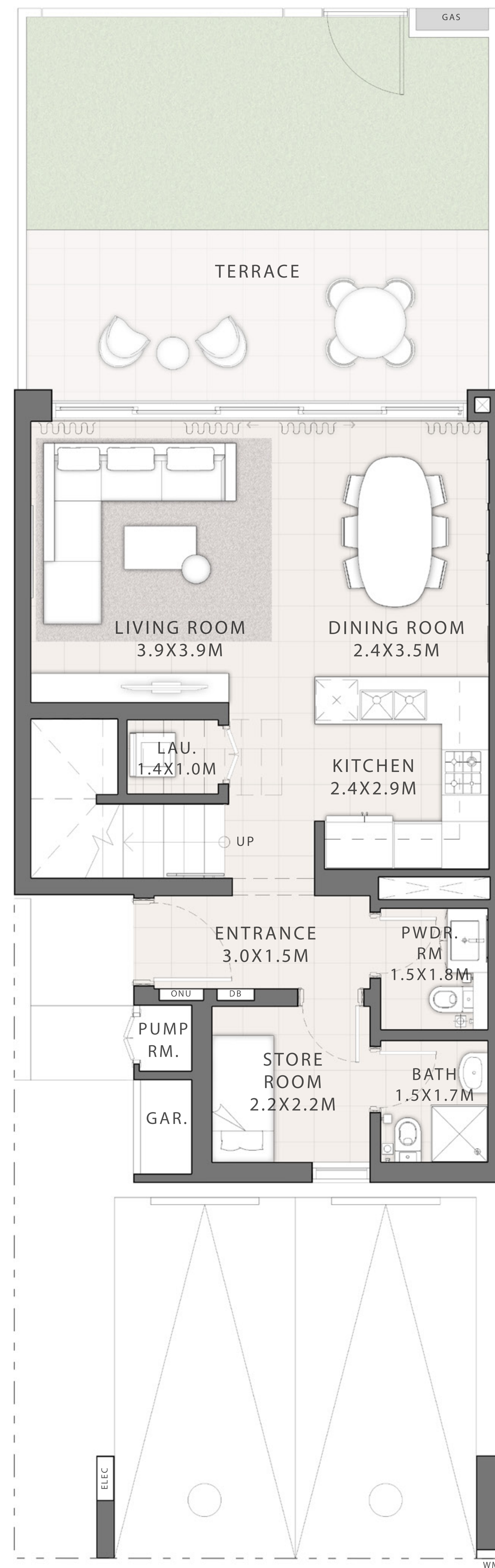
GROUND FLOOR
